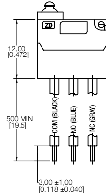
WIRE ENDS TINNED WITH ROHS COMPLIANT SOLDER
